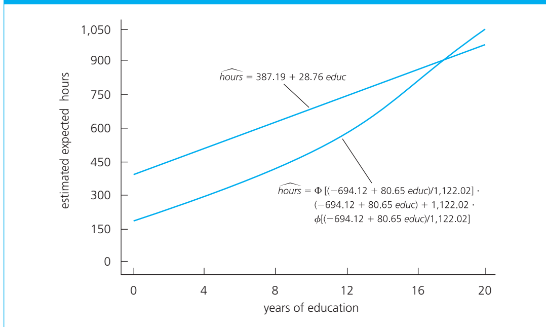
FIGURE 17.3 Estimated expected values of hours with respect to education for the linear and Tobit models.
