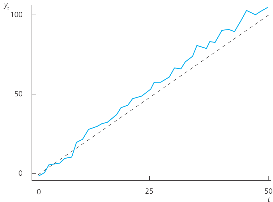
FIGURE 11.3 A realization of the random walk with drift, y_t = 2 + y_{t-1} + e_t , with y_0 = 0 , e_t s \text{Normal}(0, 9) , and n = 50 . The dashed line is the expected value of y_t , E(y_t) = 2t .
